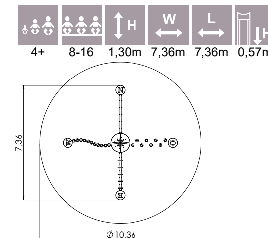
TKR001S Balance Equipment COMPASS small
