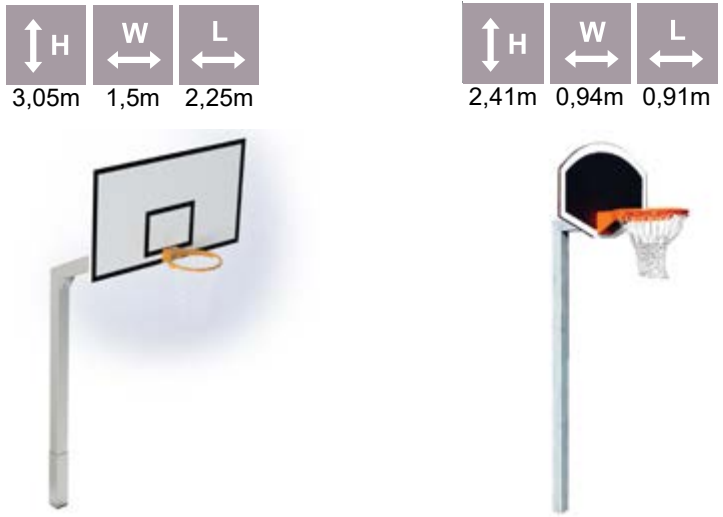
KPK04 Basketball set for children KPK09 Basketball set three heights
