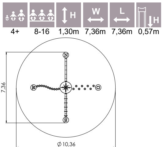
TKR001S Balance Equipment COMPASS small
