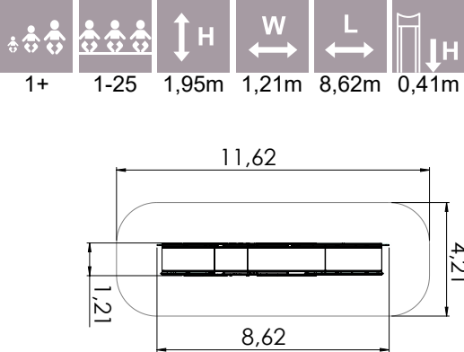
LIND3 Play equipment GREAT TIT WITH A SLOPE For kids with special needs
