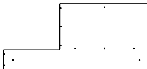
MK01 978x445mm oven back panel
