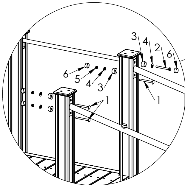
DETAIL A SCALE 1 : 15
