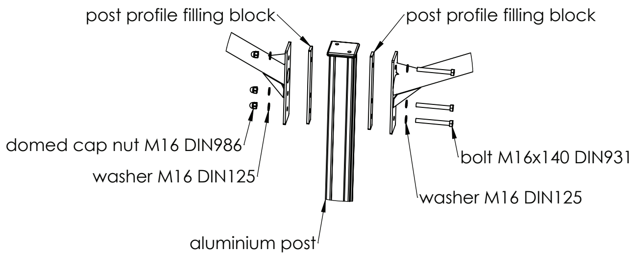
DETAIL B SCALE 1 : 15
