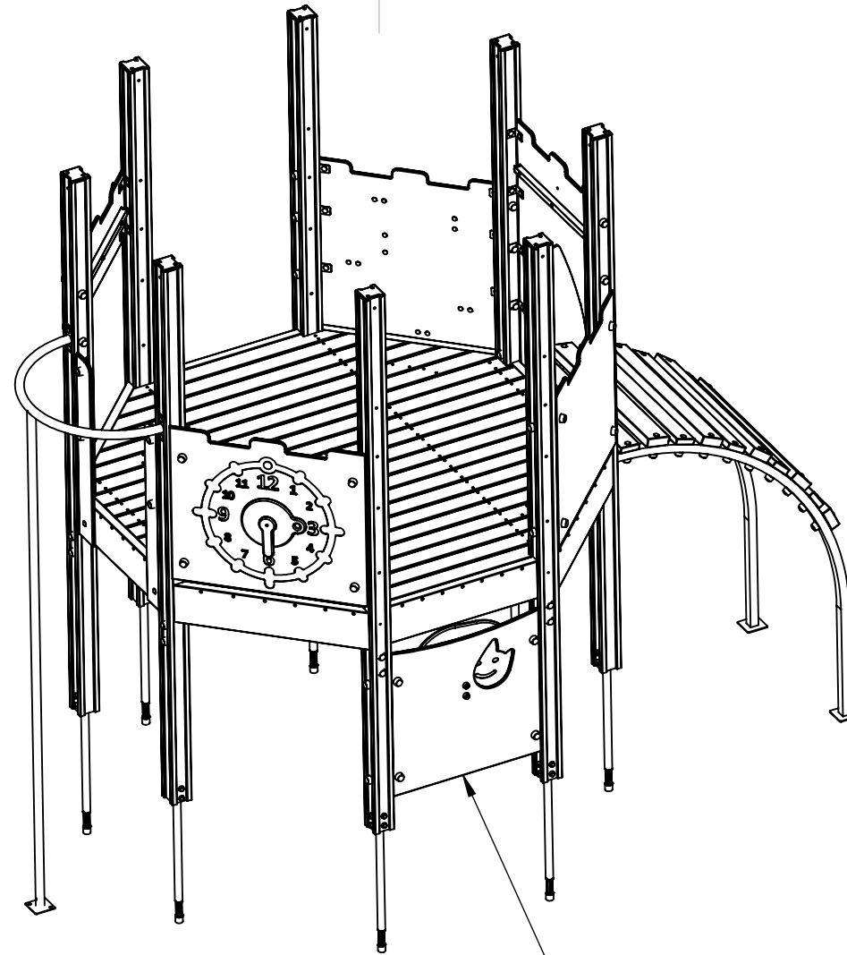
LM220-1 Emotions panel
