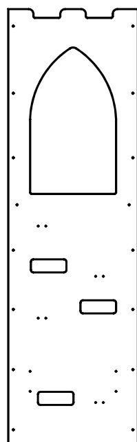
LM220-1 752x2500 panel
