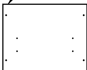
Playground rectangle panel 750x752mm with binoculars, lower hole 100mm
