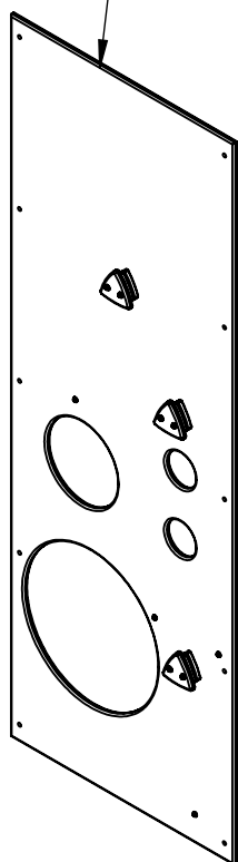
Playground rectangle panel, lower hole 85mm with clock
