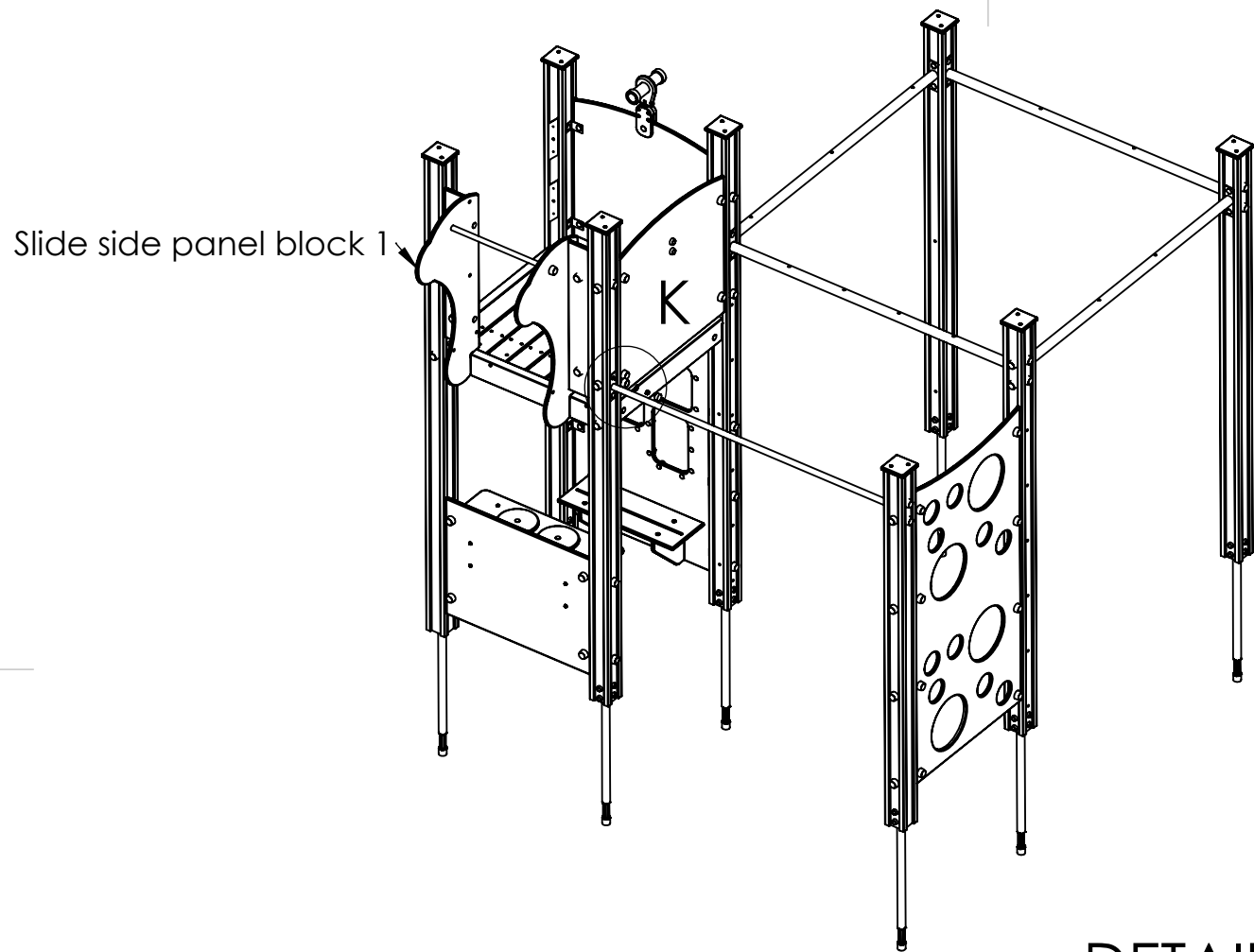
DETAIL K SCALE 1 : 7
