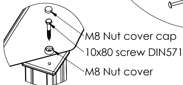
DETAIL C SCALE 1 : 7
