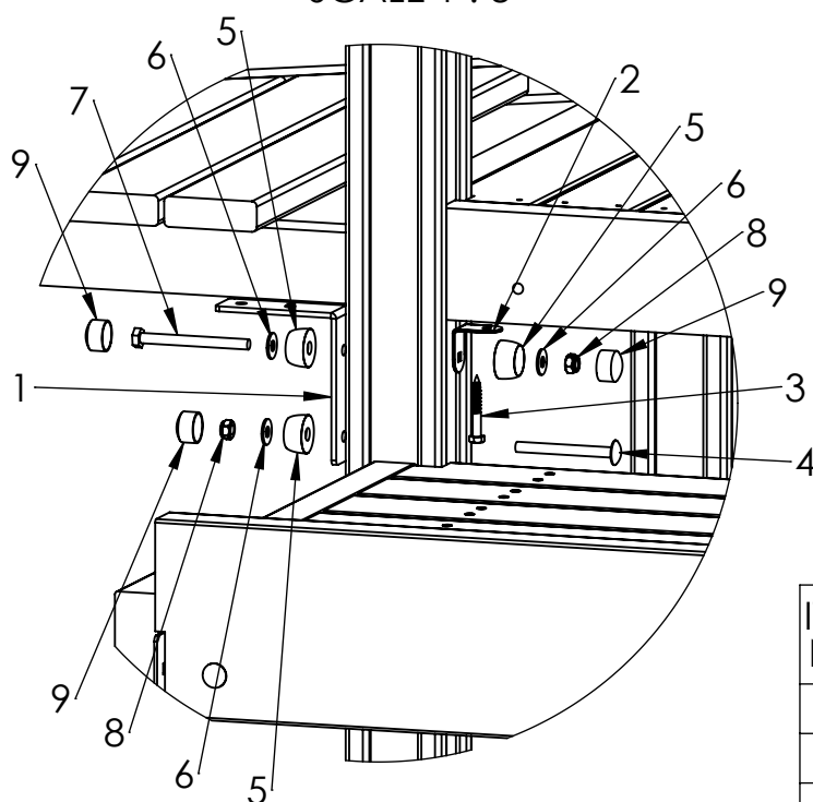
DETAIL C SCALE 1 : 8
