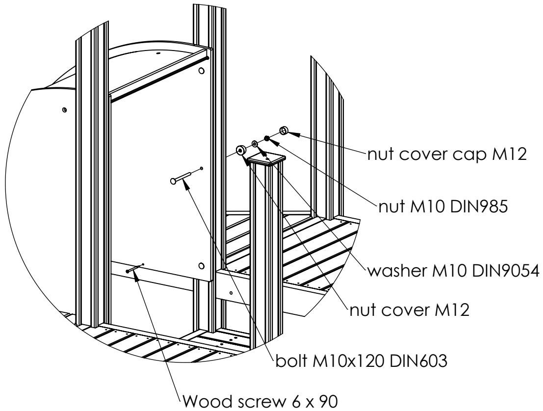
DETAIL H SCALE 1 : 15
