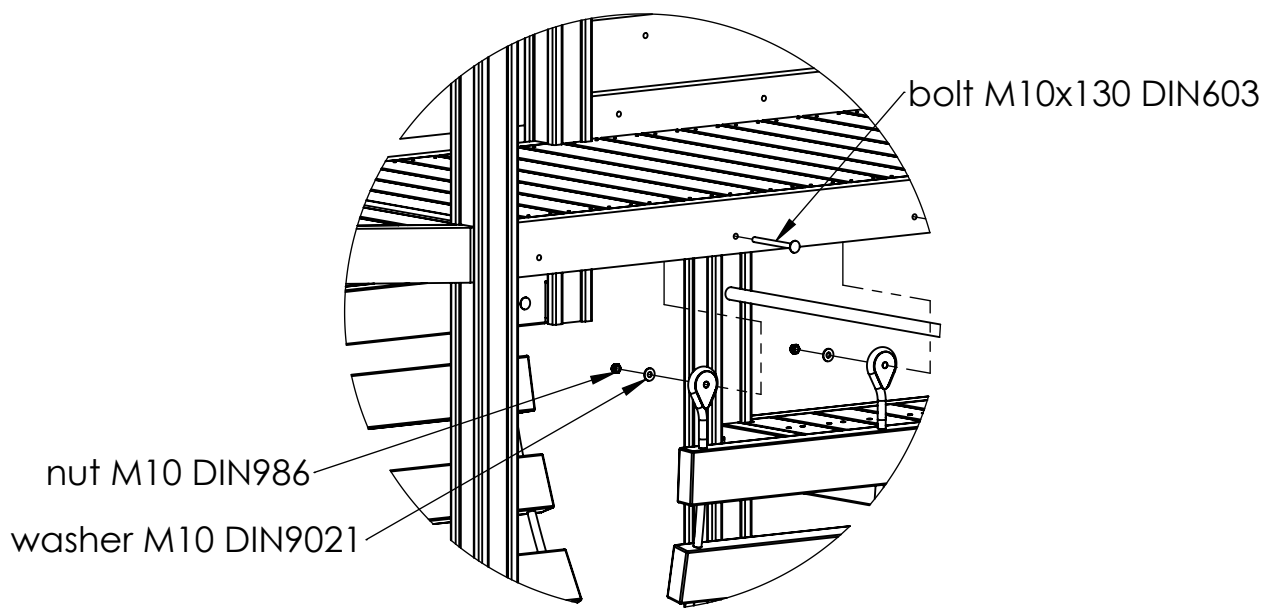
DETAIL K SCALE 1 : 15
