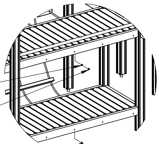
DETAIL J2 SCALE 1 : 30
