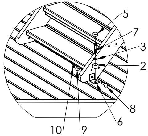
DETAIL G2 SCALE 1 : 15
