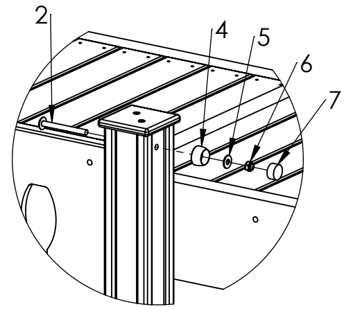
DETAIL 13 SCALE 1 : 10
