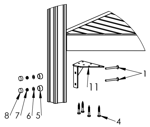
DETAIL B1 SCALE 1 : 15
