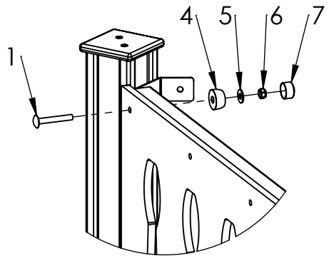
DETAIL 11 SCALE 1 : 10
